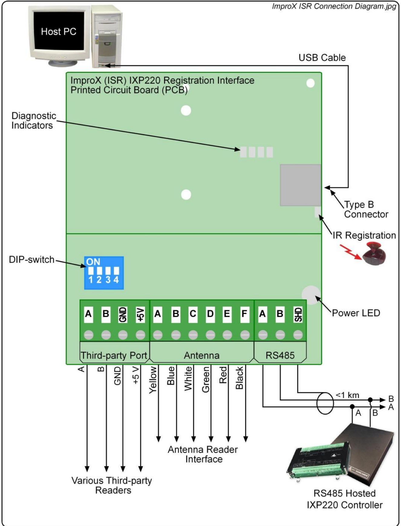
Figure 1: Typical ImproX ISR Electrical Connections
